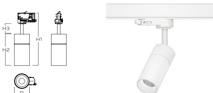
NLC-CAT14W - 4K H1 225 | H2 130 | H3 42 x D62mm
