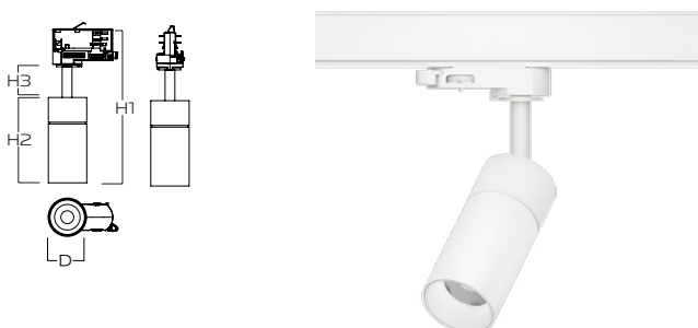
NLC-CAT11W - 4K H1 188 | H2 100 | H3 36 x D45mm
