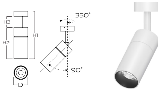
NLC-CAS14W - 4K H1 189 | H2 130 | H3 42 x D62mm
