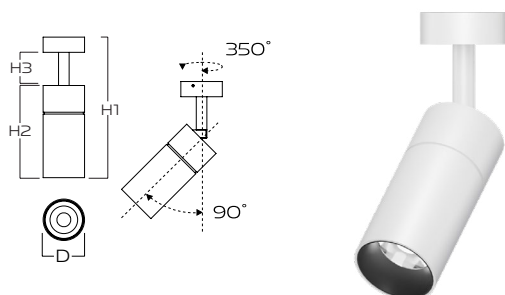
NLC-CAS11W - 4K H1 153 | H2 100 | H3 36 x D45mm
