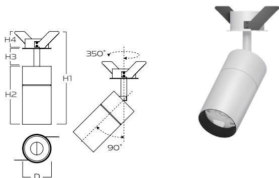
NLC-CAR24W - 4K H1 238 | H2 148 | H3 45 | H4 42 x D72mm
