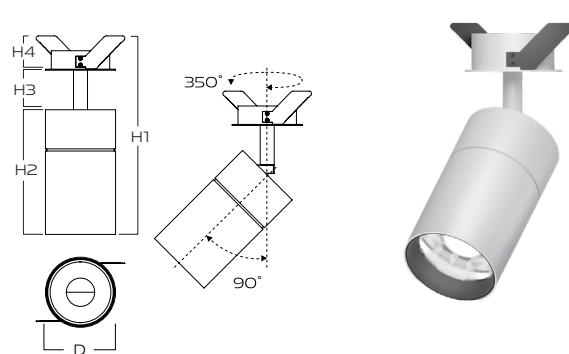
NLC-CAR36W - 4K H1 255 | H2 160 | H3 50 | H4 42 x D90mm
