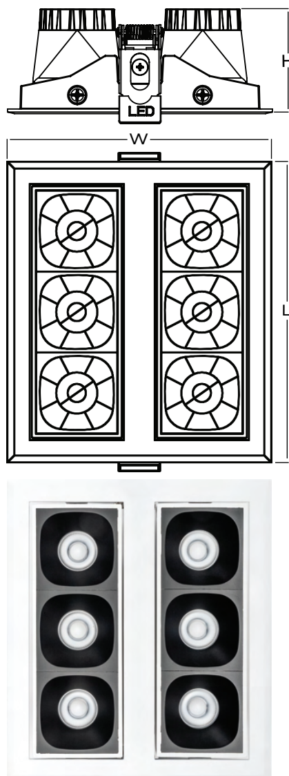
NLC-M2130W L130 x W114 x H45mm Cut size: 122x102mm
