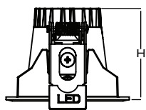
NLC-MI5W L60 x W60 x H45mm Cut size: 52x52mm
