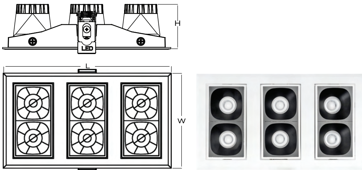
NLC-M3130W L168 x W95 x H45mm Cut size: 160x87mm
