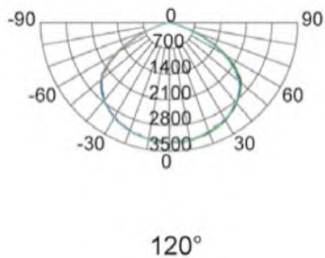
Photometric Data
